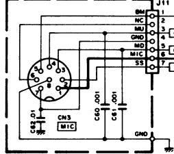
SWITCH UNIT (X41-1610-00) (D/14)
