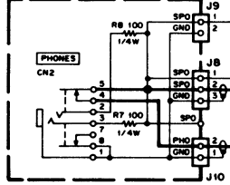
SWITCH UNIT (X41-1610-00) (G/14)
