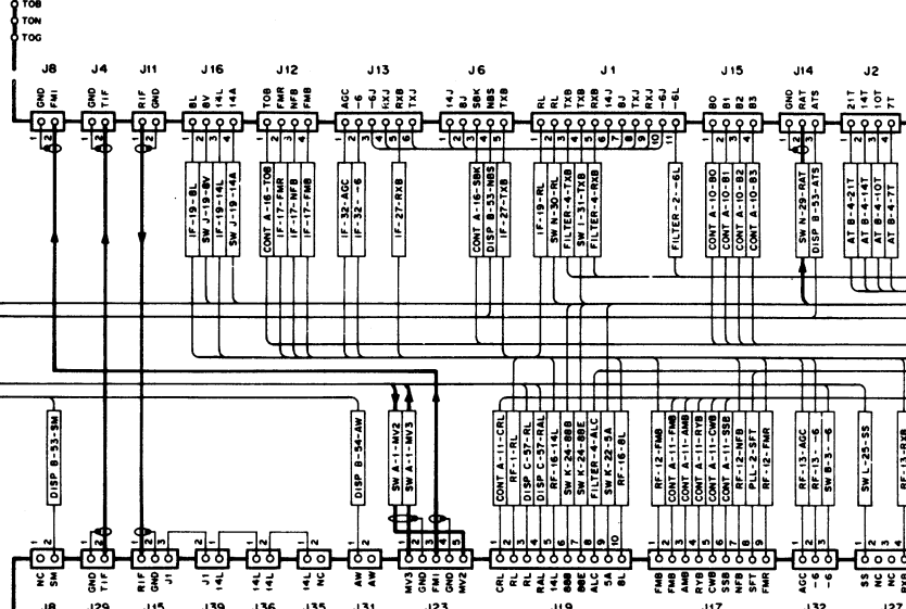
RF UNIT (X44-1680-00)
