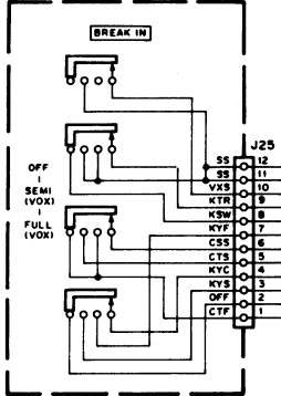
SWITCH UNIT (X41-1610-00) (L/14)
