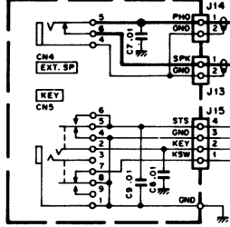
SWITCH UNIT (X41-1610-00) (G/14)
